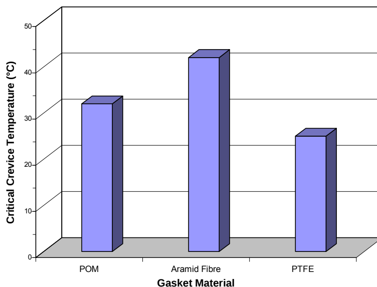
FIGURE 2 Critical crevice temperature at +600mV SCE for 6%Mo stainless steel with different gasket materials (Ref 7)
